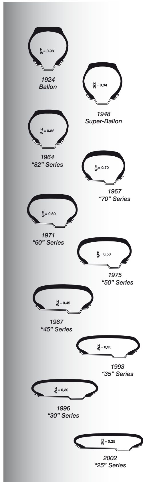
H:W - Height / Width aspect ratio of a tyre (also called 'series')
